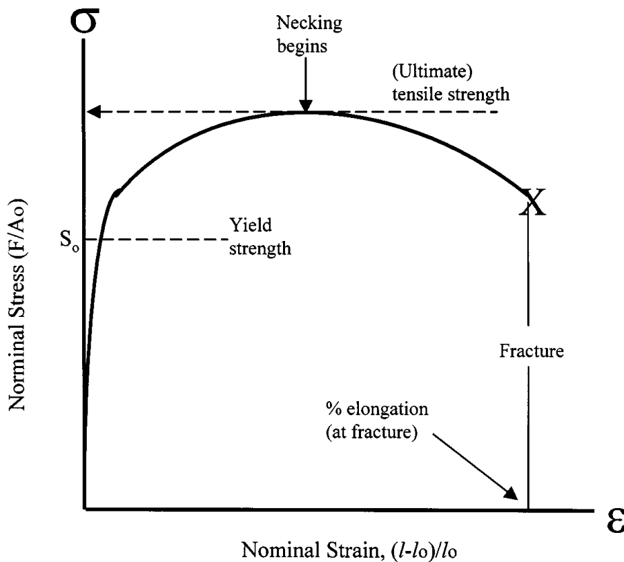
FIGURE 12.1.3 Typical engineering stress–strain curve for a metal.
