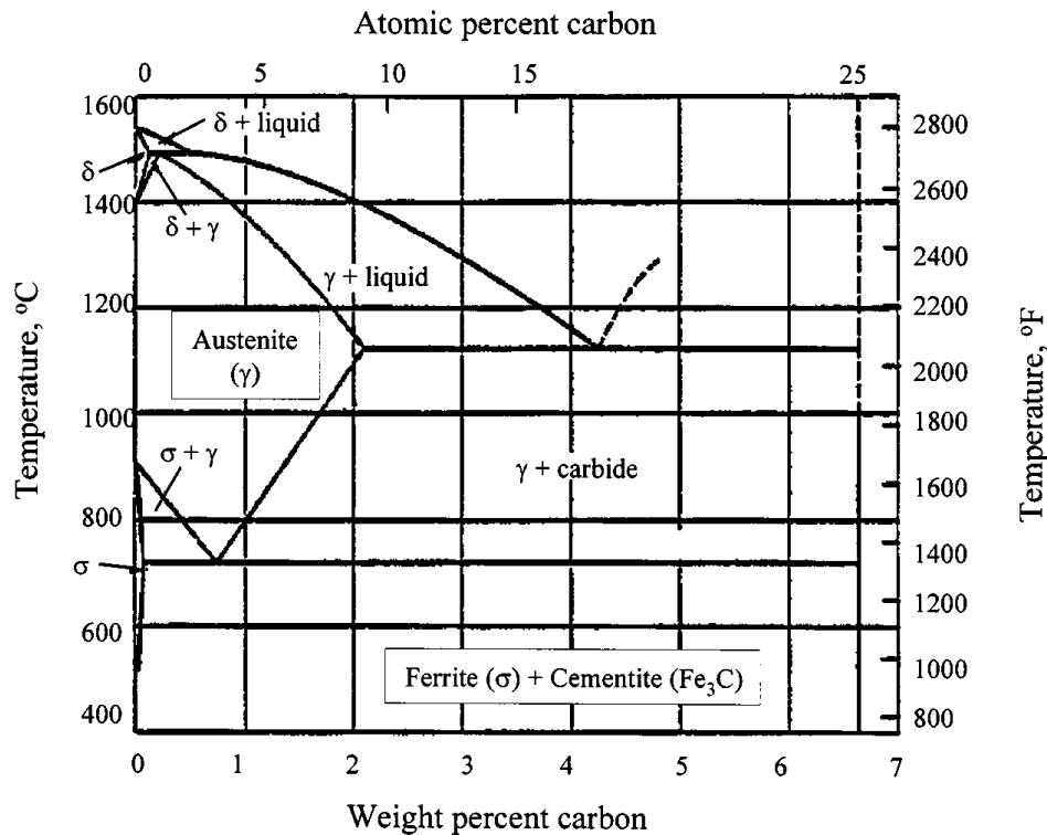
FIGURE 12.1.8 Iron–carbon phase diagram relevant for steel. The steel composition range is from about 0.02 to 1.00 w/o carbon. Steel strengthening treatments require heating into the austenite region (above the A_{c3} ) and then quenching.
