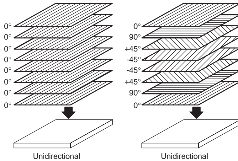
FIGURE 12.6.3 The basic concept of composite laminate.
