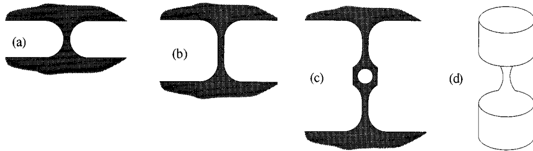
FIGURE 11.8.39 Monolithic flexural bearings.
