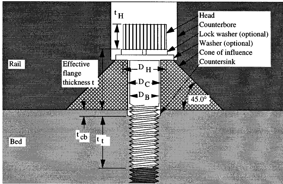
FIGURE 11.8.31 Typical components of a bolted assembly.
