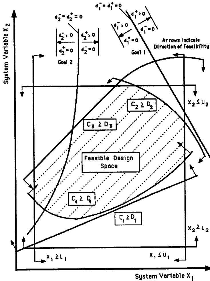
FIGURE 11.10.18 The compromise DSP.
