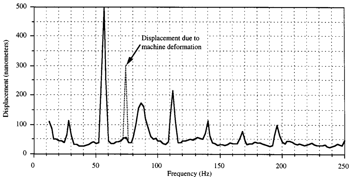
FIGURE 11.8.12 FFT of grinding spindle error motion.
