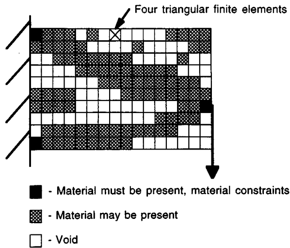
FIGURE 11.10.6 Typical design domain.
