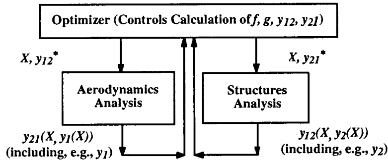
FIGURE 11.10.16 Single-SAND-NAND formulation.
