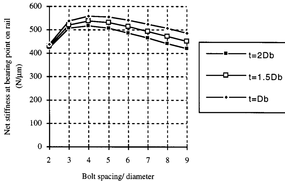
FIGURE 11.8.33 Relationships among stiffness and bolt spacing.
