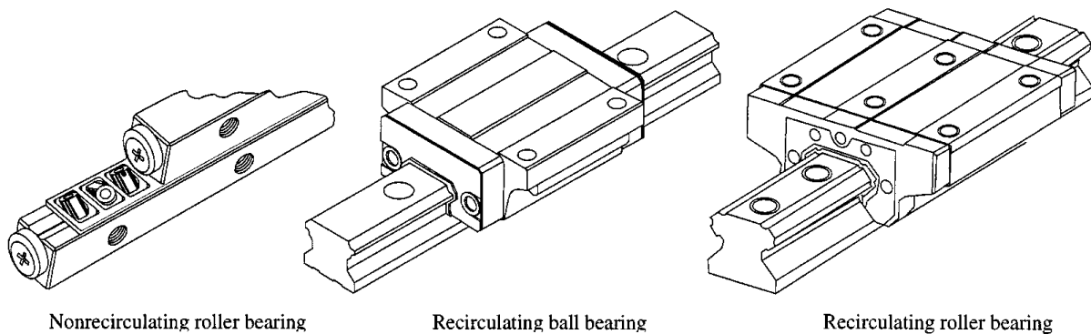
FIGURE 11.8.38 Typical linear rolling element bearing configurations.
