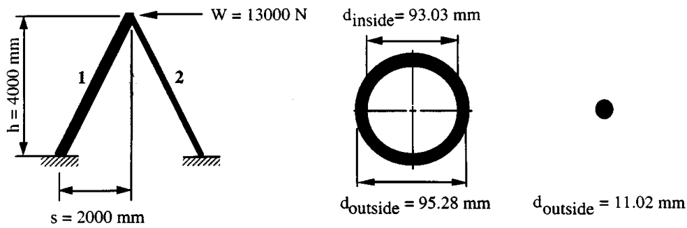
FIGURE 11.10.4 (a) Configuration of the optimized truss design.
