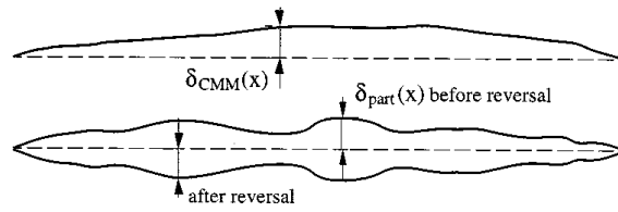
FIGURE 11.8.3 Illustration of the principal of reversal.
