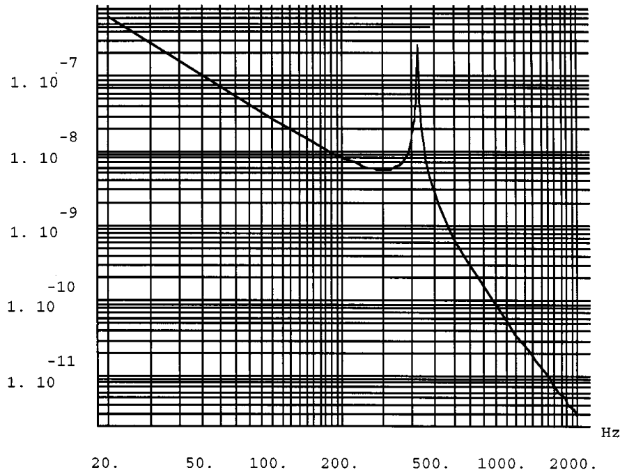
FIGURE 11.8.19 Frequency response of a ballscrew-driven system.
