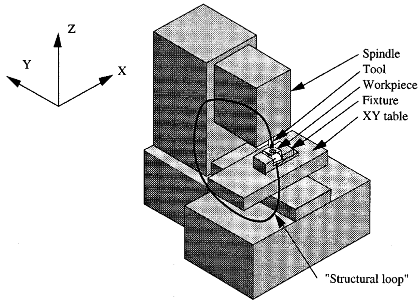
FIGURE 11.8.25 Structural loop in an open-frame machine tool.
