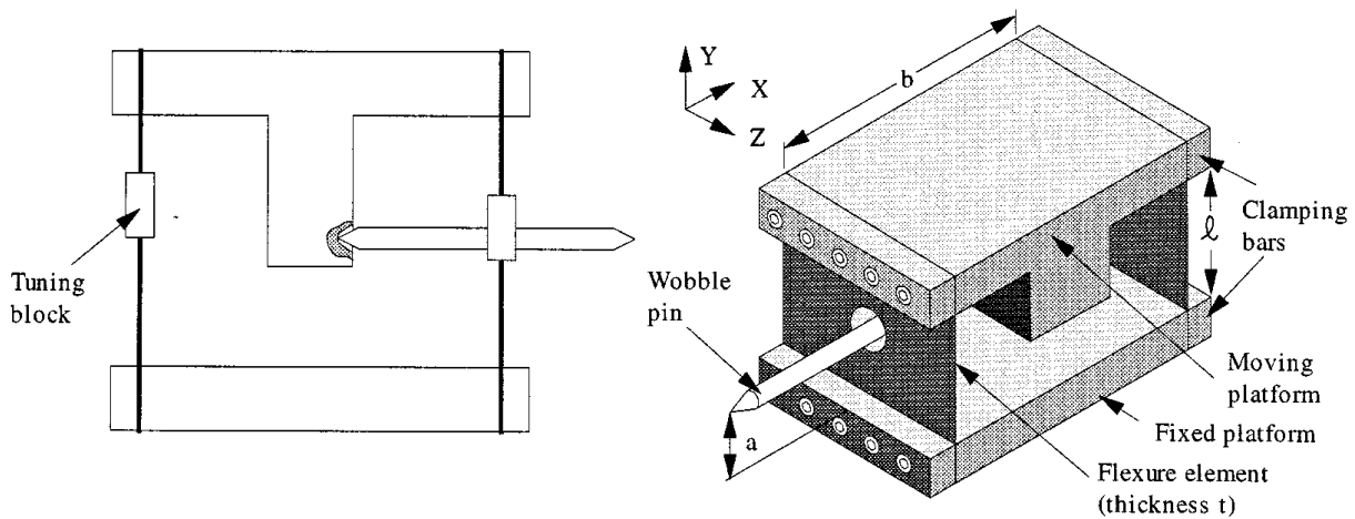
FIGURE 11.8.40 Clamped (blade) flexure.
