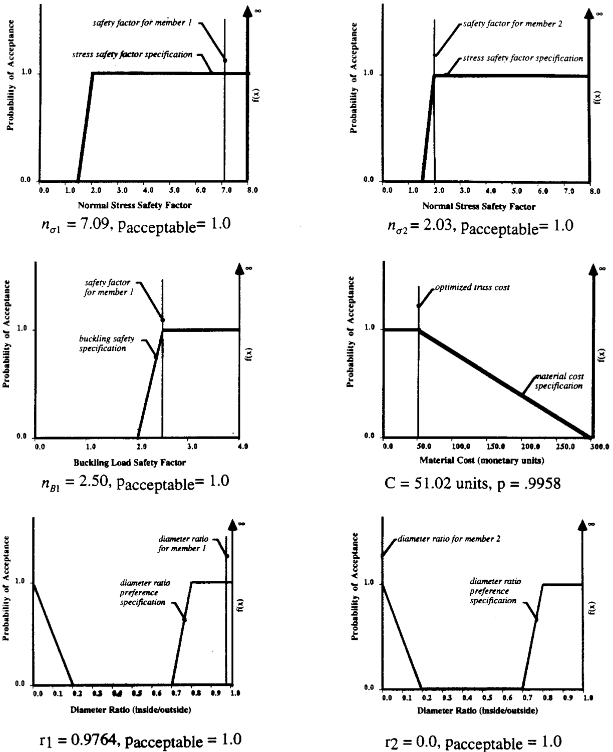
FIGURE 11.10.4 (b) Comparison of truss performance variables to design specifications.
