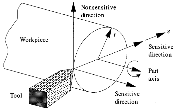
FIGURE 11.8.2 Illustration of sensitive directions.
