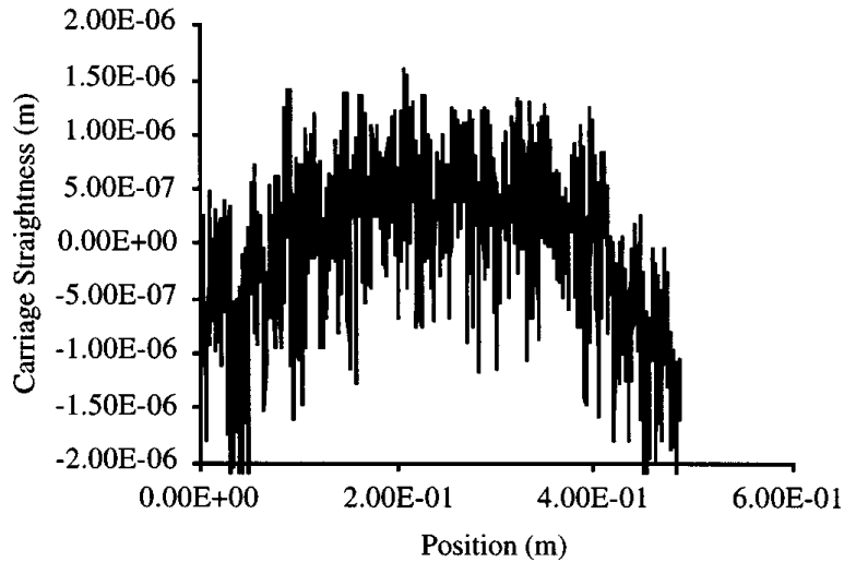
FIGURE 11.8.8 Strightness of a linear motion system.
