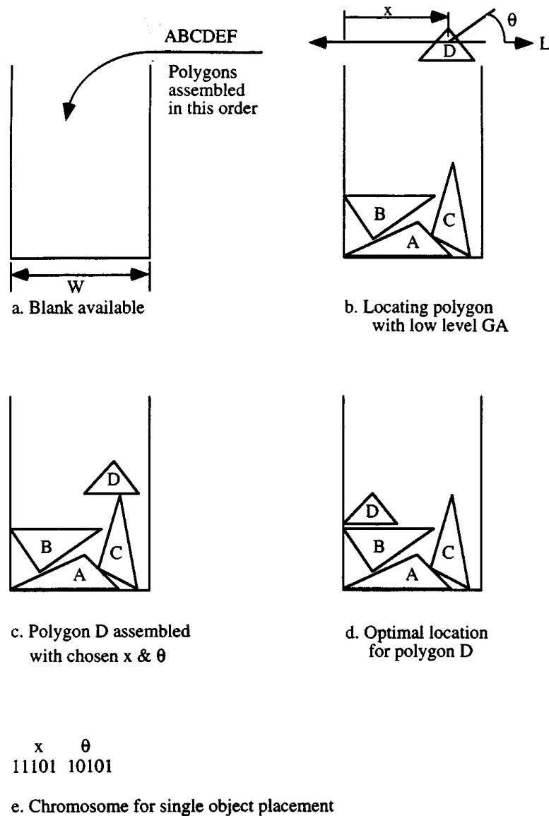
FIGURE 11.10.10 Lower-level GA for hierarchical shape packing.
