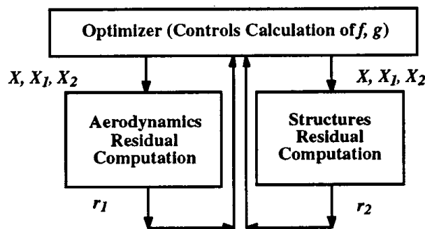
FIGURE 11.10.15 Single-SAND-SAND formulation.
