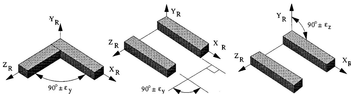
FIGURE 11.8.14 Orthogonality and horizontal and vertical parallelism errors.
