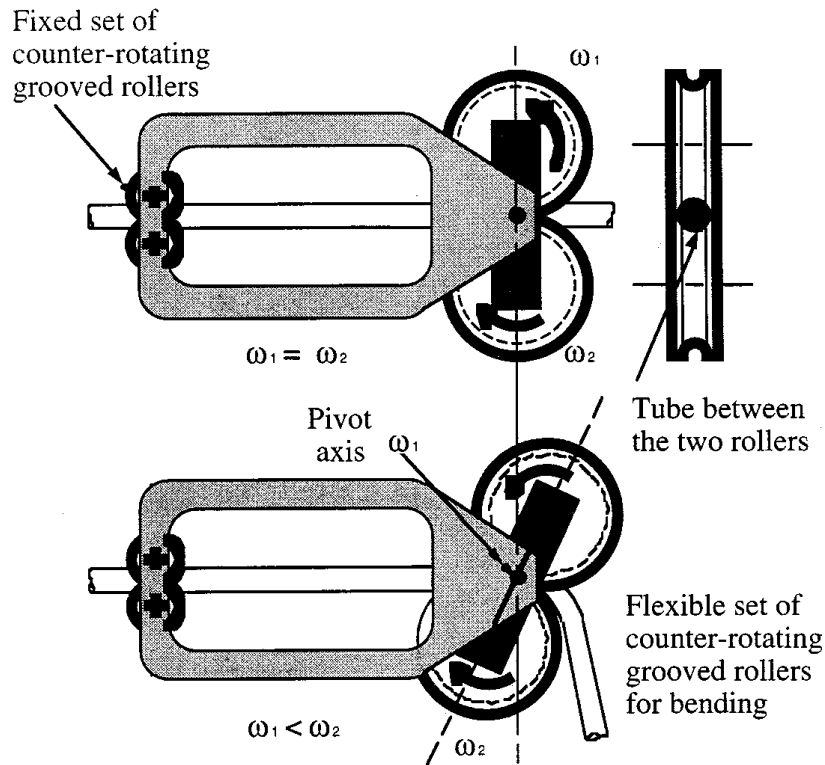
FIGURE 11.4.2 Concept for tube bending.
